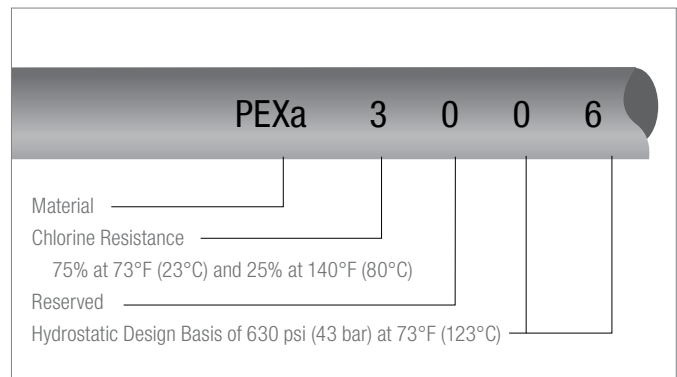
Fig. 4.2: Example RAUPEX O 2 Barrier Pipe Material Designation Code
