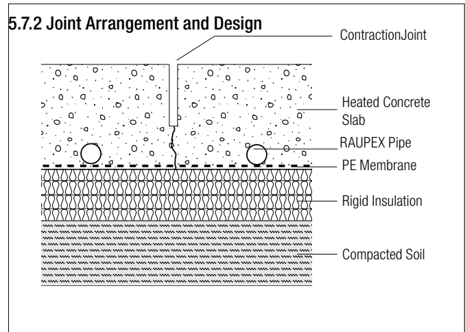
Fig. 5.3: Contraction joint
