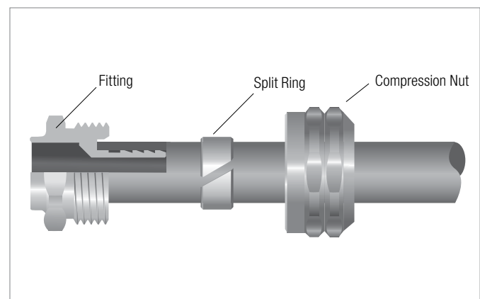
Fig. 4.6: Adapter connection to copper pipe
