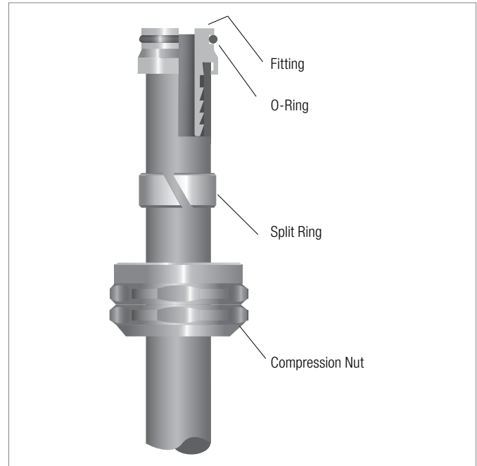
Fig. 4.5: R20 connection to manifold
