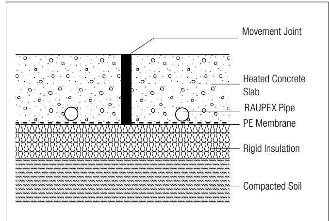
Fig. 5.2: Movement joint
